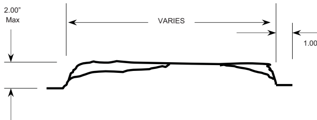
Formliner sheet size: 48" x 116-1/2"
