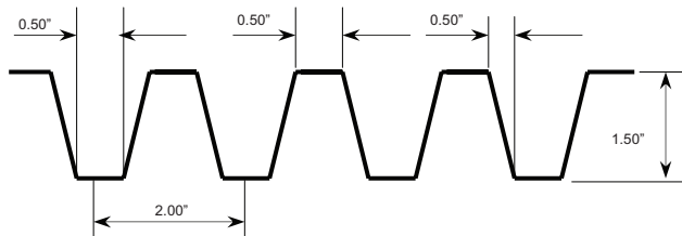
Trapezoid 1102 - 1-1/2" Deep 2" O.C.
