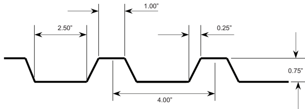
Trapezoid 1110 - 3/4" Deep 4" O.C.
