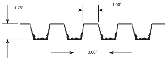
Fractured 1401 - 1-3/4" Deep 3" O.C. 1" Rib
